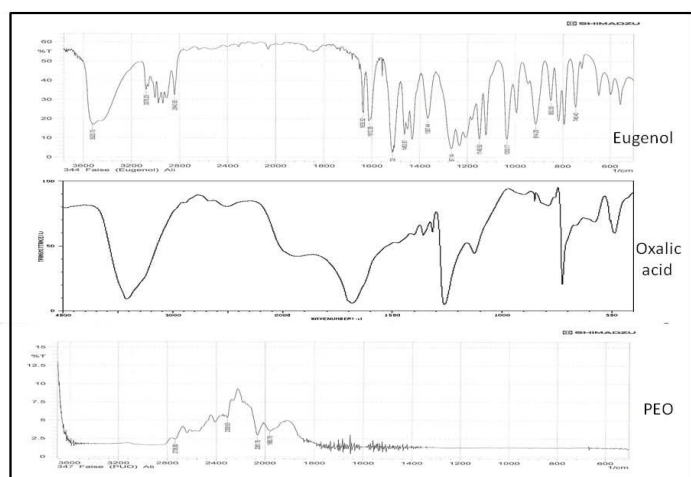
Figure 3: The FTIR Spectra for Eugenol, Oxalic Acid 12 and PEO
