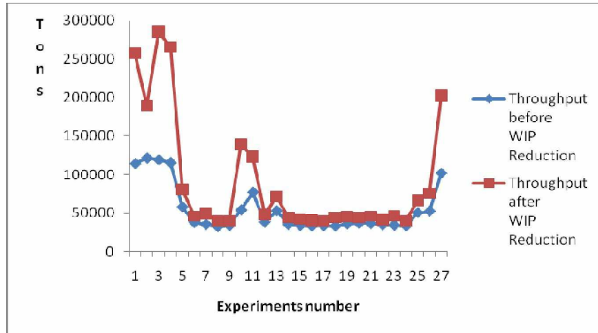
Figure 2: Throughput Before & After WIP Reduction
