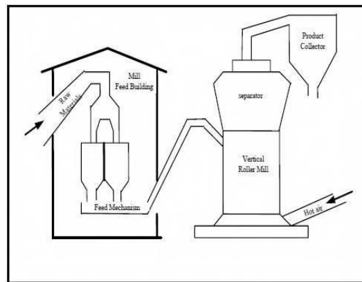
Figure 1: The Dry Raw Milling Process
