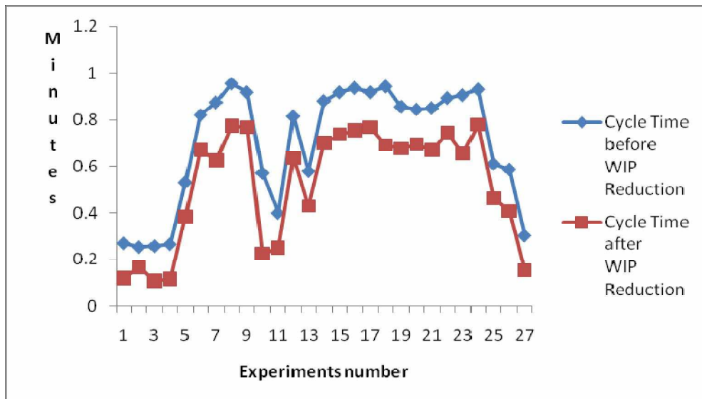
Figure 4: Cycle Time Before & After WIP Reduction
